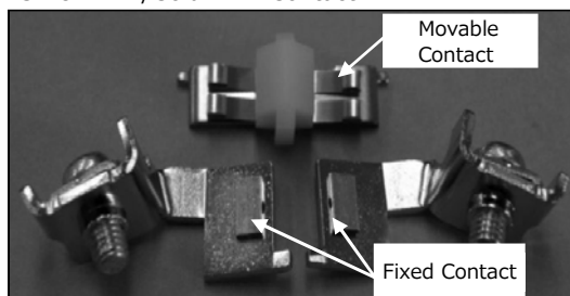
Silver Twin/Gold Twin Contact
