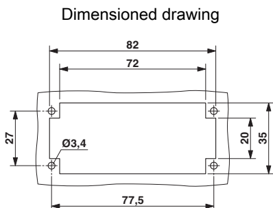
Mounting cutout when used without housing
