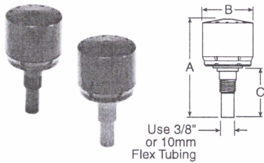
Automatic Drain GRP-95-973, GRP-95-981
