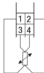
Potentiometer 4 wire sensor
