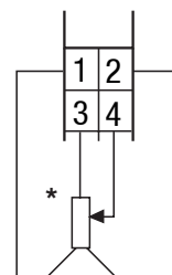
Potentiometer 4 wire sensor
