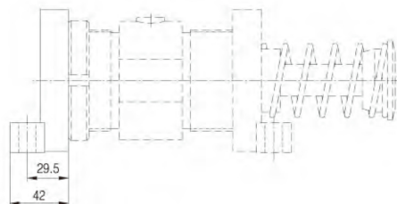
Clevis Mount Set (LA85-CMS)
