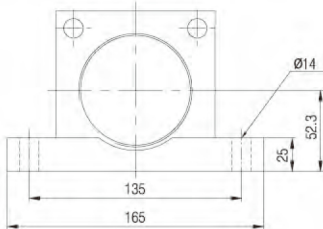
Foot Mount (LA85-FM)
