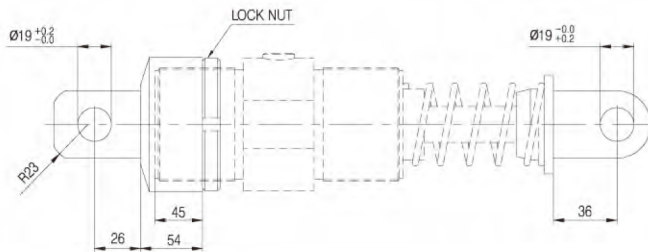
Clevis Mount Set (LA85-CMS)
