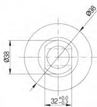
Cylinder Clevis (LA85-CC)
